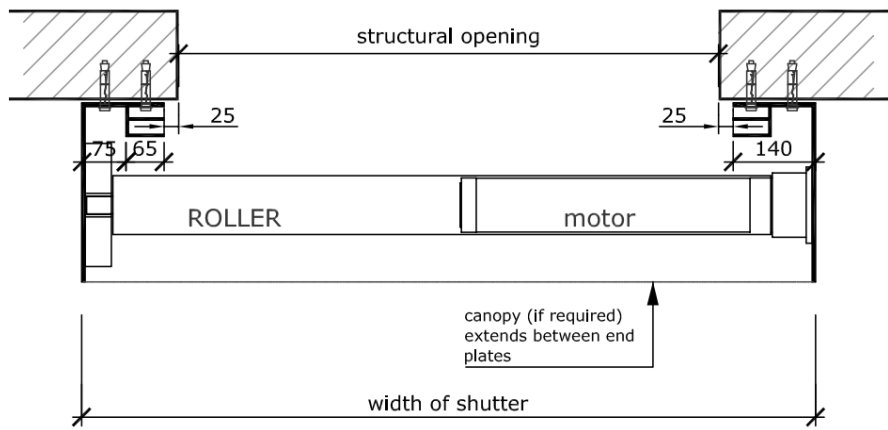
Plan views: Reveal Fix (above) and Face Fix (below)
