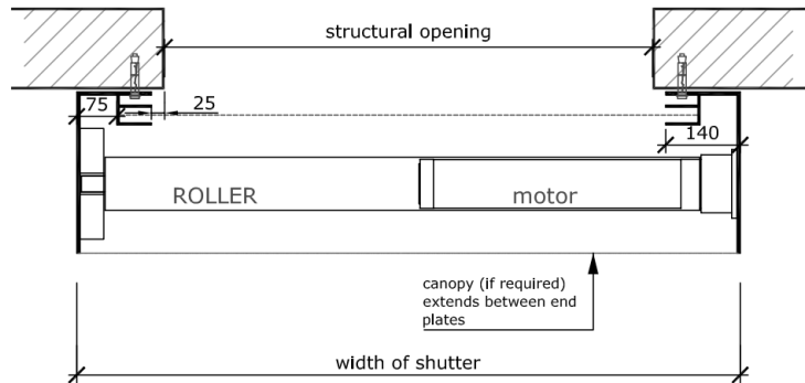
Plan view face fix (above) and reveal fix (below)
